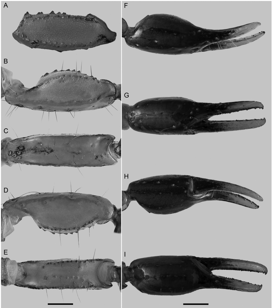
FIGURE 18. Maaykuyak waueri (Gertsch and Soleglad, 1972), ♂ (CNAN 2062), dextral pedipalp femur (A), patella (B–E) and chela (F–I). A, B, F. Dorsal aspect. C, G. Retrolateral aspect. D, H. Ventral aspect. E, I. Prolateral aspect. Scale bars = 0.25 mm.
