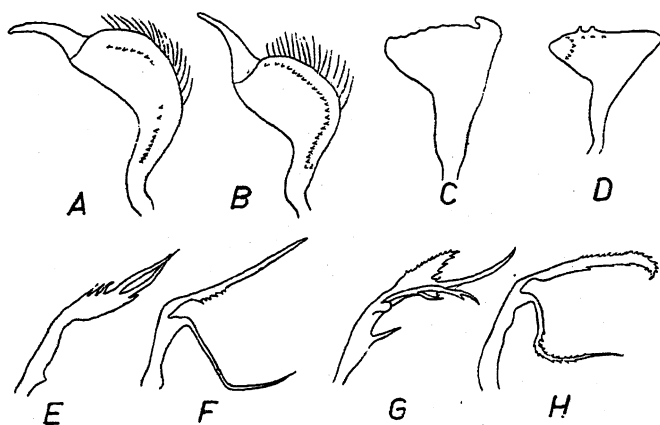
Fig. 2. Genitalia of male. A = left paramere of O. ericetorum FALL. (60 times); B = id. of O. carneae ssp. nov.; C = right paramere of O. ericetorum FALL. (60 times); D = id. of O. carneae ssp. nov.; E + F = appendages of the vesica of O. ericetorum FALL. (42 times); G + H = id. of O. carneae ssp. nov.
