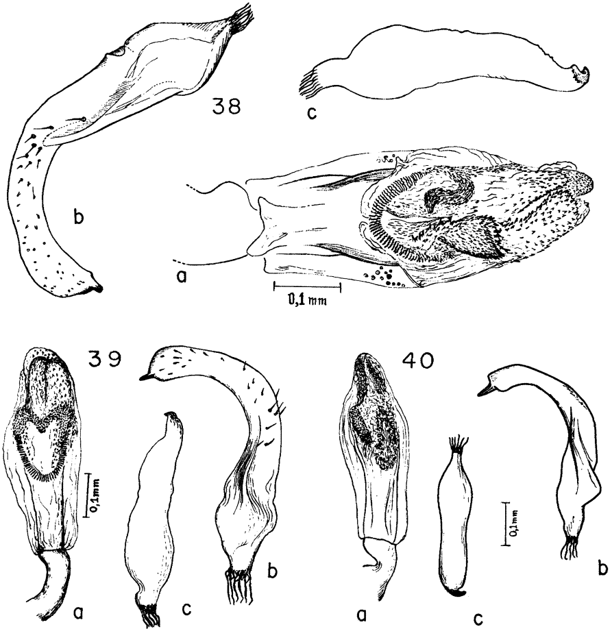
FIGURES 38-40. Creontiades species: a, Aedeagus; b, Left clasper; c, Right clasper. Figure 38. C. fernandinus Carvalho, new species; figure 39. C. fuscus Barber; figure 40. C. willowisi Van Duzee.
