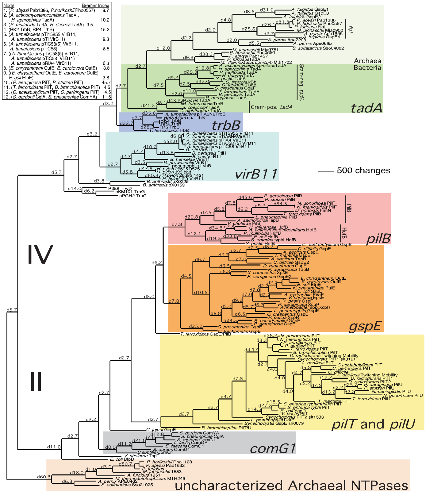
Fig. 1. A phylogenetic tree of putative NTPase genes of type II/IV secretion systems constructed with maximum parsimony algorithms. Gene subfamilies are designated by colored boxes, and subgroupings, by vertical lines. Archaeal and Bacterial divisions in the tadA gene subfamily are shown in two shades of green. The numbers on branches are Bremer indices of the nodes at the end of the designated branch (see Methods ). Bremer indices for some organisms did not fit onto the tree and are supplied in the box in the upper left corner. Accession numbers for all genes are listed on the web site http://cpmncnet.columbia.edu/dept/figurski .
