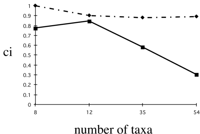
Figure 3 Plot of the consistency index of chromosomal inversion partition (dotted line) and the DNA sequence partition (solid line) when forced to fit the parsimony tree versus the number of taxa in the data set. The melanogaster species group analysis has eight taxa, the virilis species group analysis has 12 taxa, the picture wing species group has 35 taxa and the repleta species group has 54 taxa.
