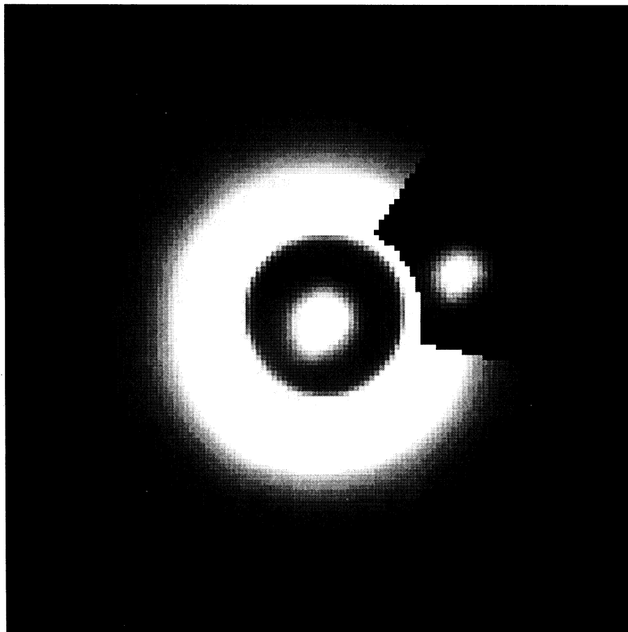
FIG. 1.—1993 I_C image of Gl 105A obtained with the Adaptive Optics Coronagraph. The field is 14''.5 \times 14''.5 , with north at the top and east to the left. The 2''.15 radius occulting mask is slightly transparent and reveals the core of the occulted star's seeing disk. Part of the seeing disk has been subtracted to reveal the companion, Gl 105C, located 3''.30 from Gl 105A at P.A. 287^\circ . The companion has an I_C magnitude of 12.6.
